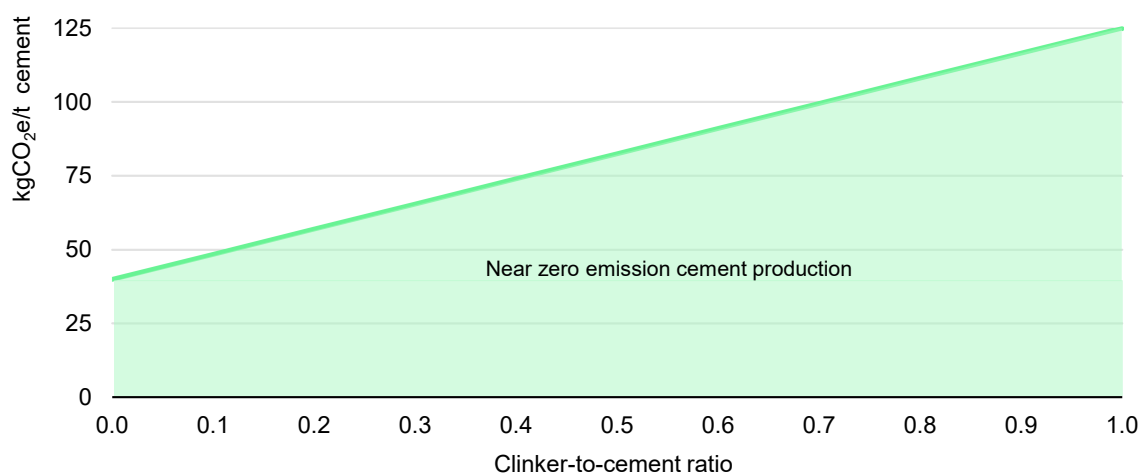
Figure 3.5 Near zero emission cement production threshold as a function of the clinker-to-cement ratio
