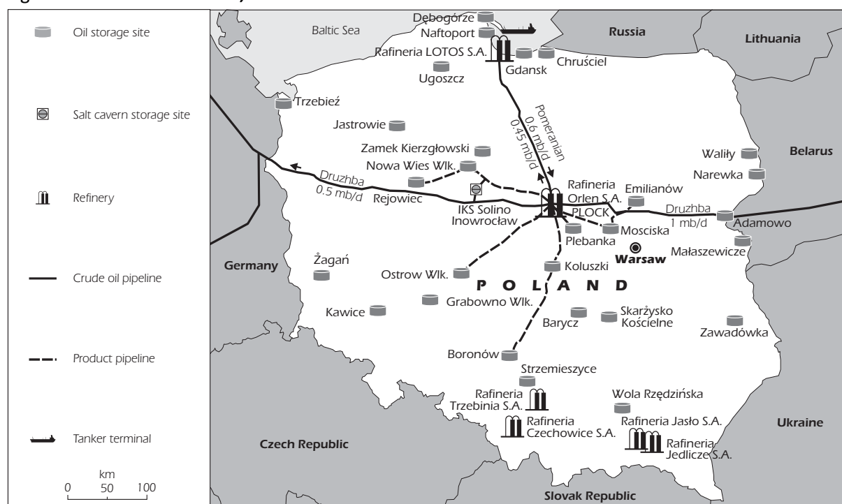
Figure 36. Oil infrastructure, 2010
