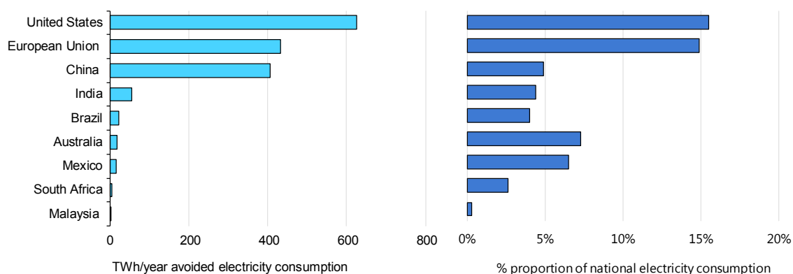
Figure 1 EES&L programme-related annual electricity savings, 2018
