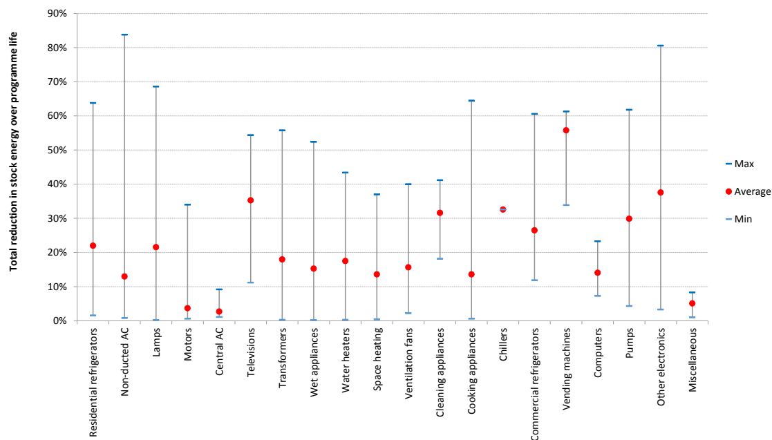
Figure 9 Appliance energy savings from EES&L programmes over life of programmes
