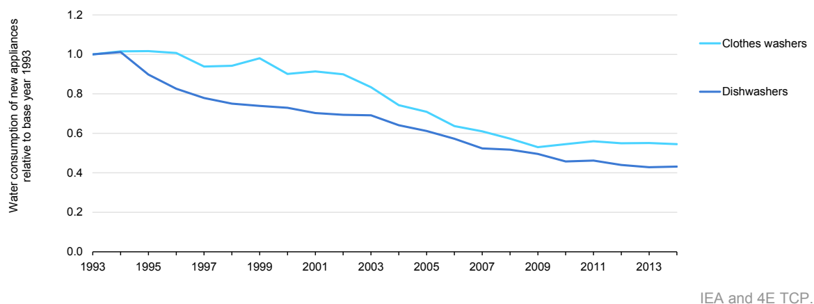
Figure 14 Changes in water consumption of new clothes washers and dishwashers in Australia, 1993-2014
