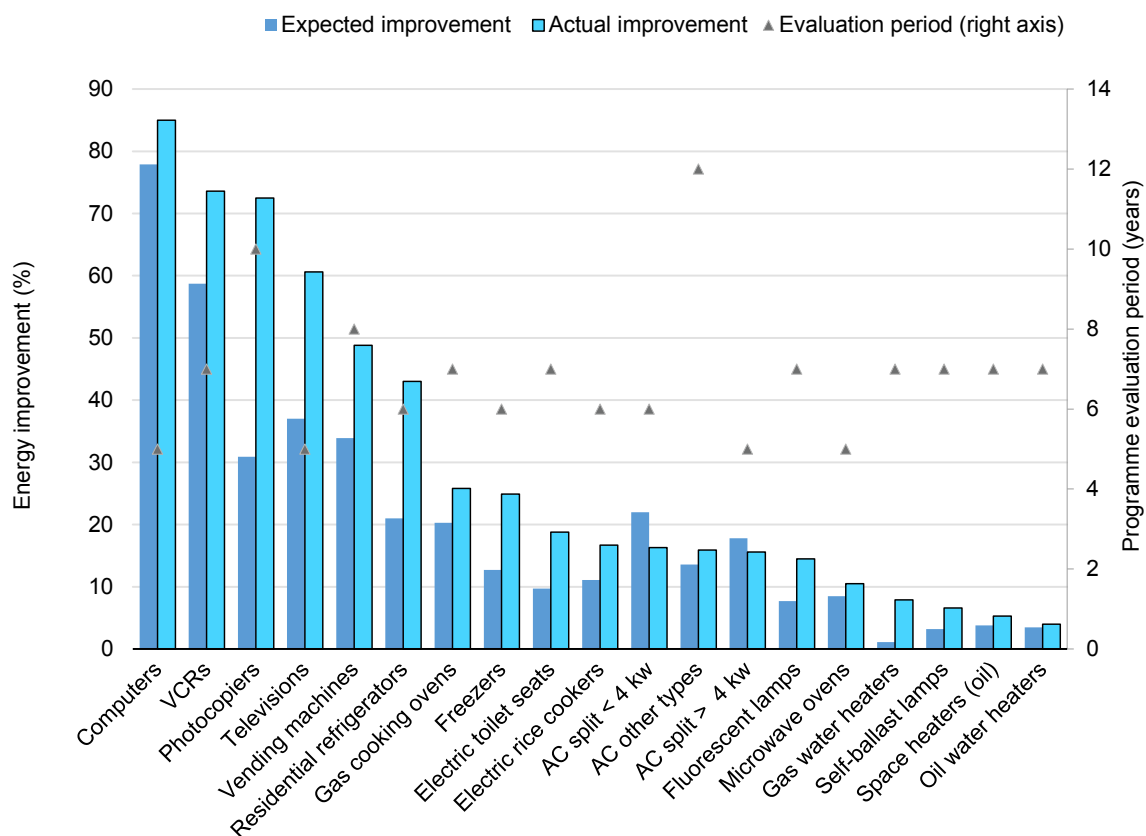
Figure 11 Expected versus delivered improvements of the Japanese Top Runner Programme
