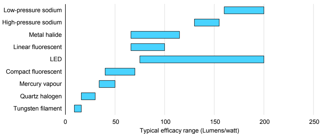
Figure 10 Typical range of efficacy for different lighting technologies
