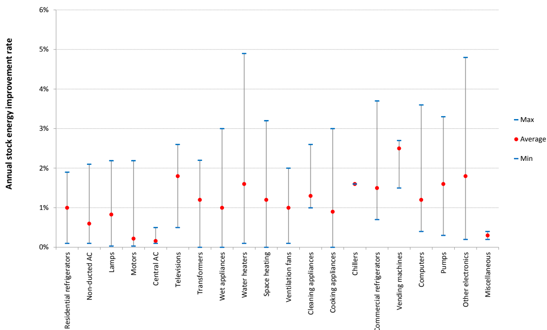
Figure 8 Annual reduction in stock average energy consumption from EES&L programmes
