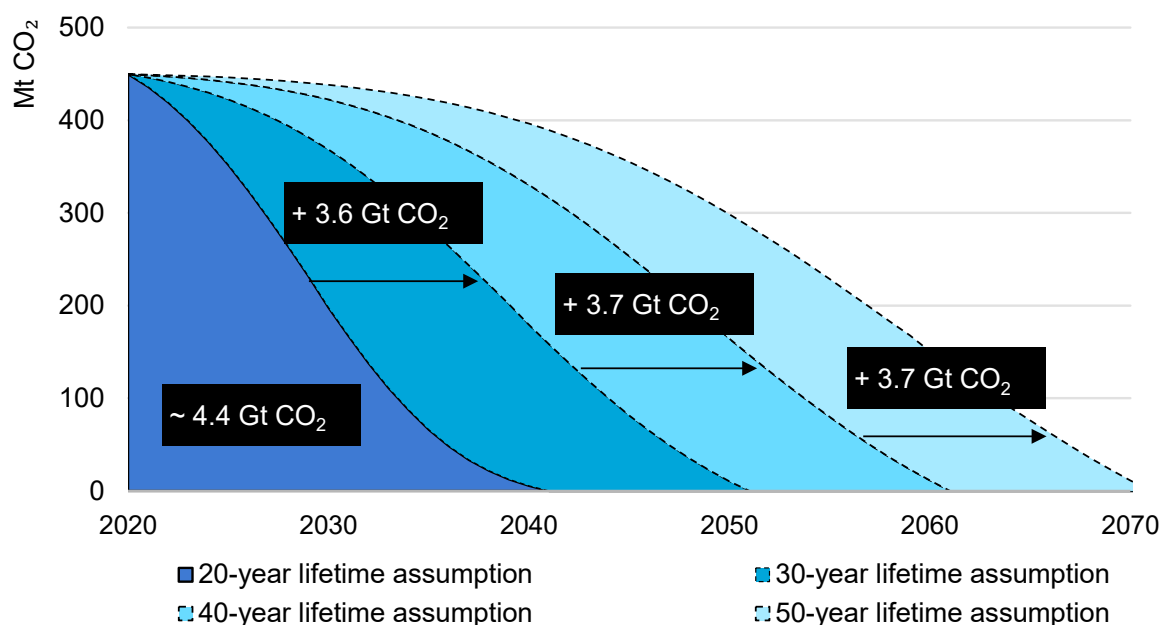
Figure 1.9 Projected emissions from existing ammonia plants under different lifetime assumptions
